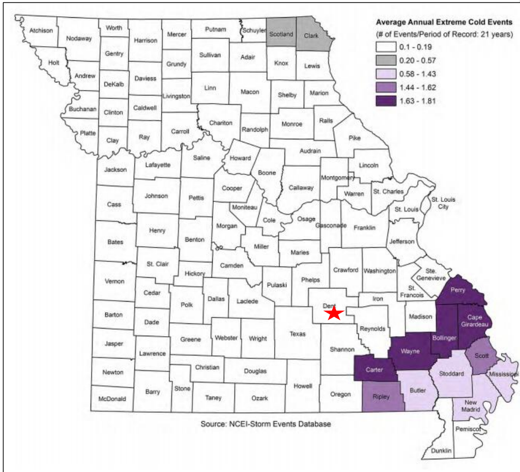
Figure 3.29. Average Annual Occurrence for Extreme Cold
