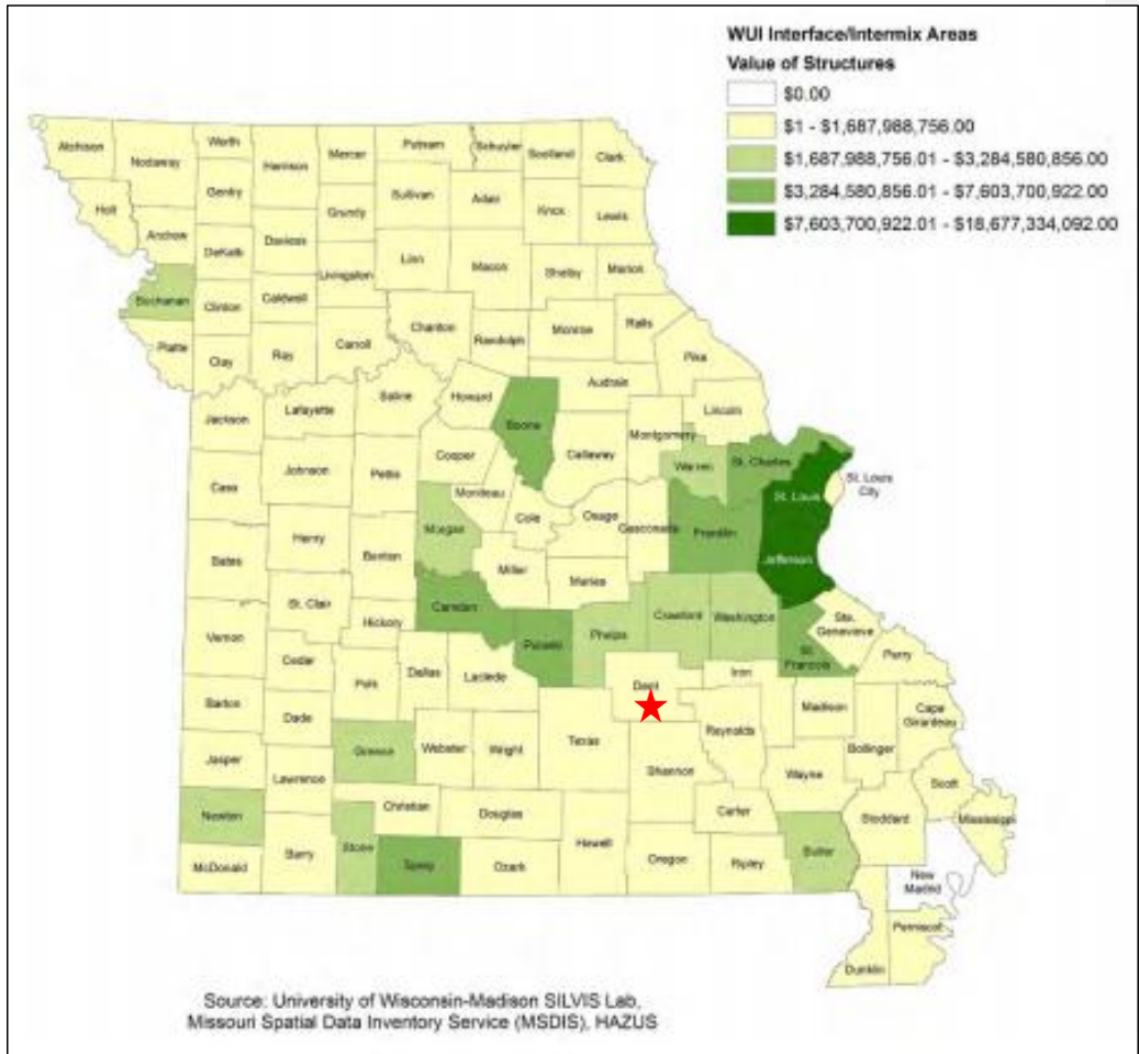
Figure 3.73. Value of Structures in the WUI Interface and Intermix Areas
