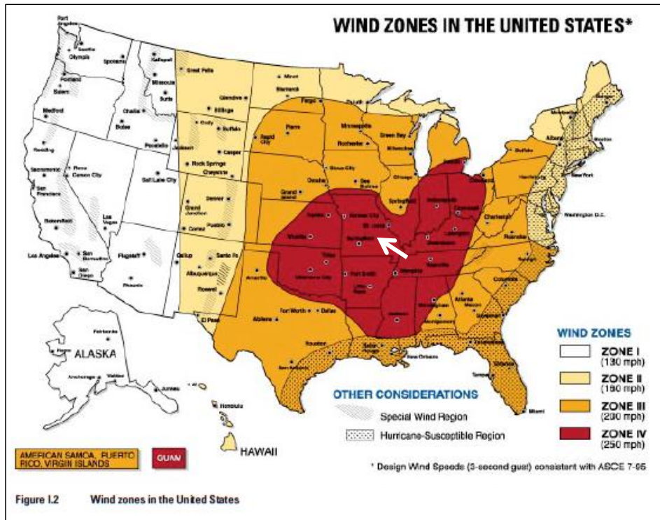
Figure 3.52. Wind Zones in the United States
