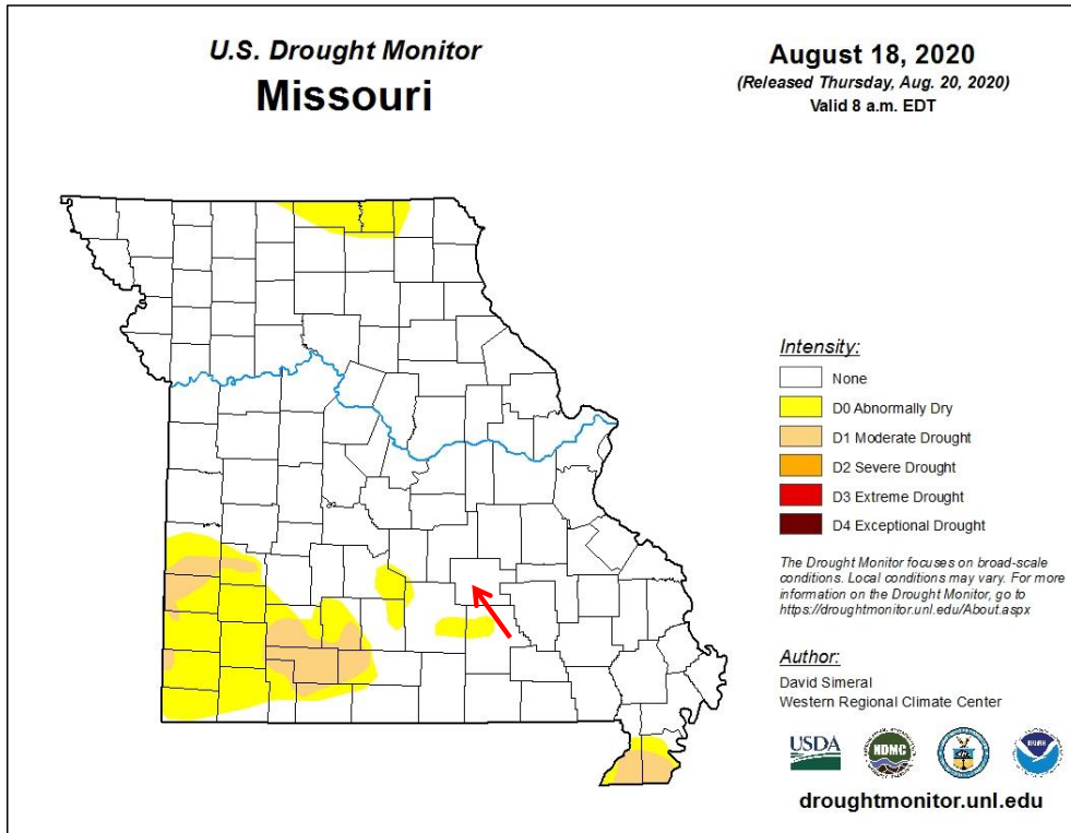
Figure 3.12. U.S. Drought Monitor Map of Missouri on August 18, 2020
