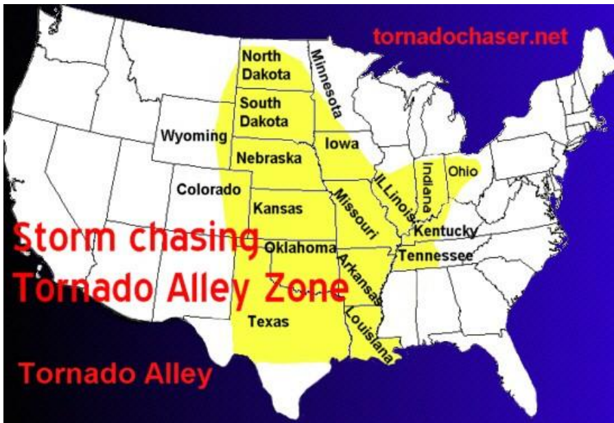
Figure 3.64. Tornado Alley in the U.S.
