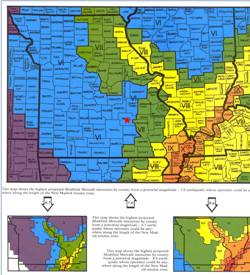
Figure 3.18. Impact Zones for Earthquake Along the New Madrid Fault
