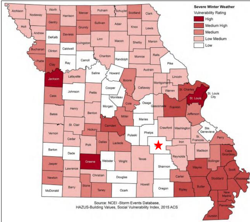
Figure 3.61. Vulnerability Summary for Severe Winter Weather
