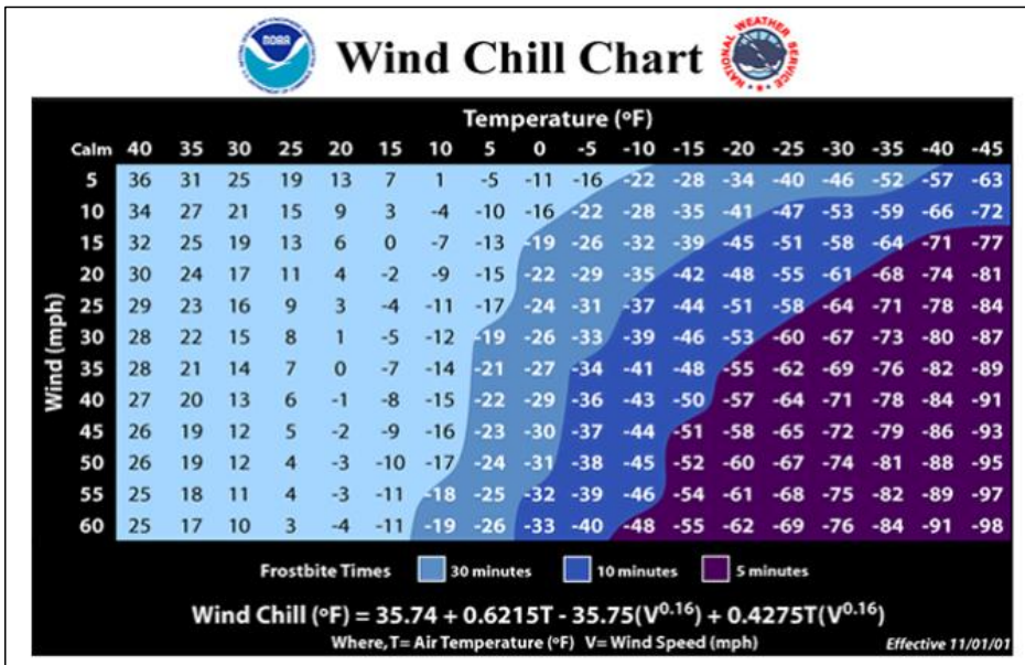
Figure 3.26. Wind Chill Chart
