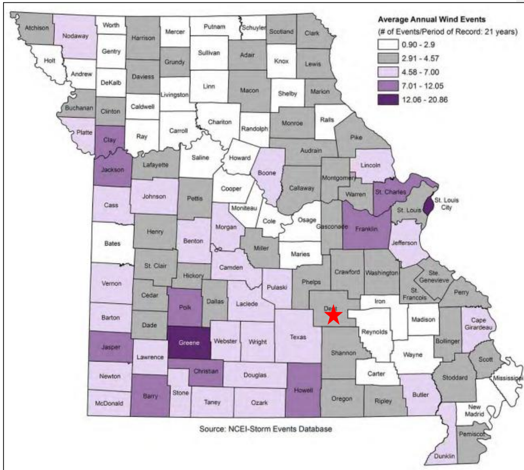
Figure 3.54. Average Annual High Wind Events (40 MPH and Higher)
