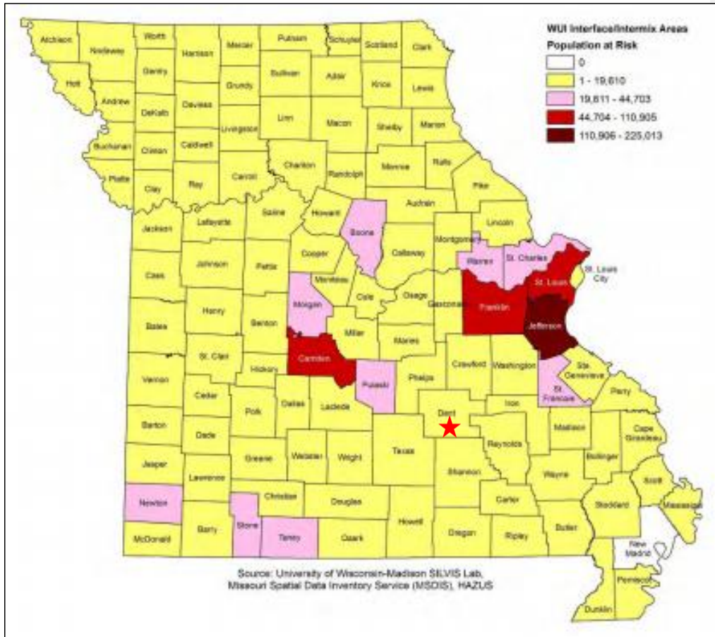
Figure 3.74. Population at Risk to Wildfire in WUI Interface and Intermix Areas
