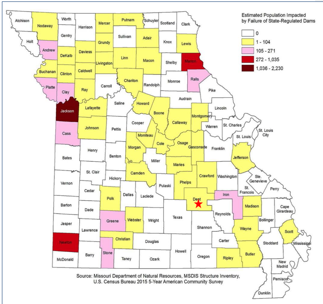
Figure 3.11. Estimated Population Exposure to Failure of State-regulated Dams
