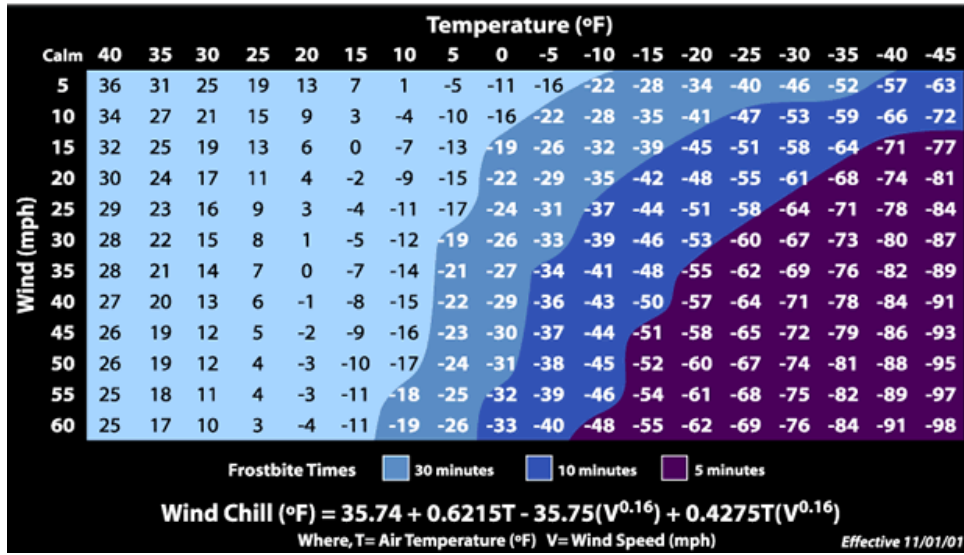
Figure 3.59. Wind Chill Chart
