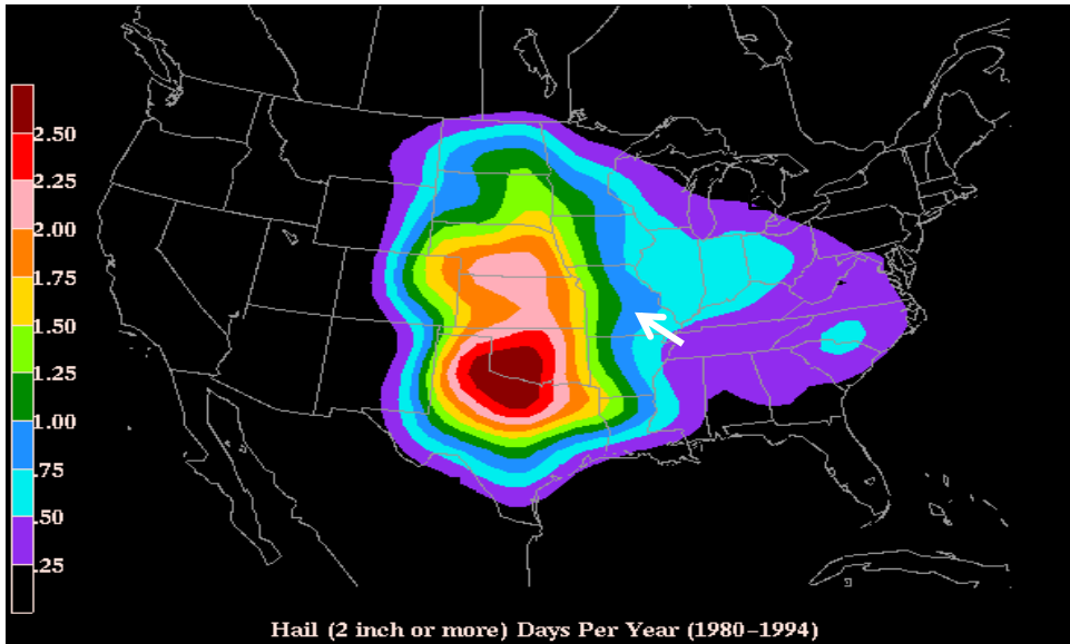
Figure 3.53. Annual Hailstorm Probability (2" diameter or larger), 1980 - 1994
