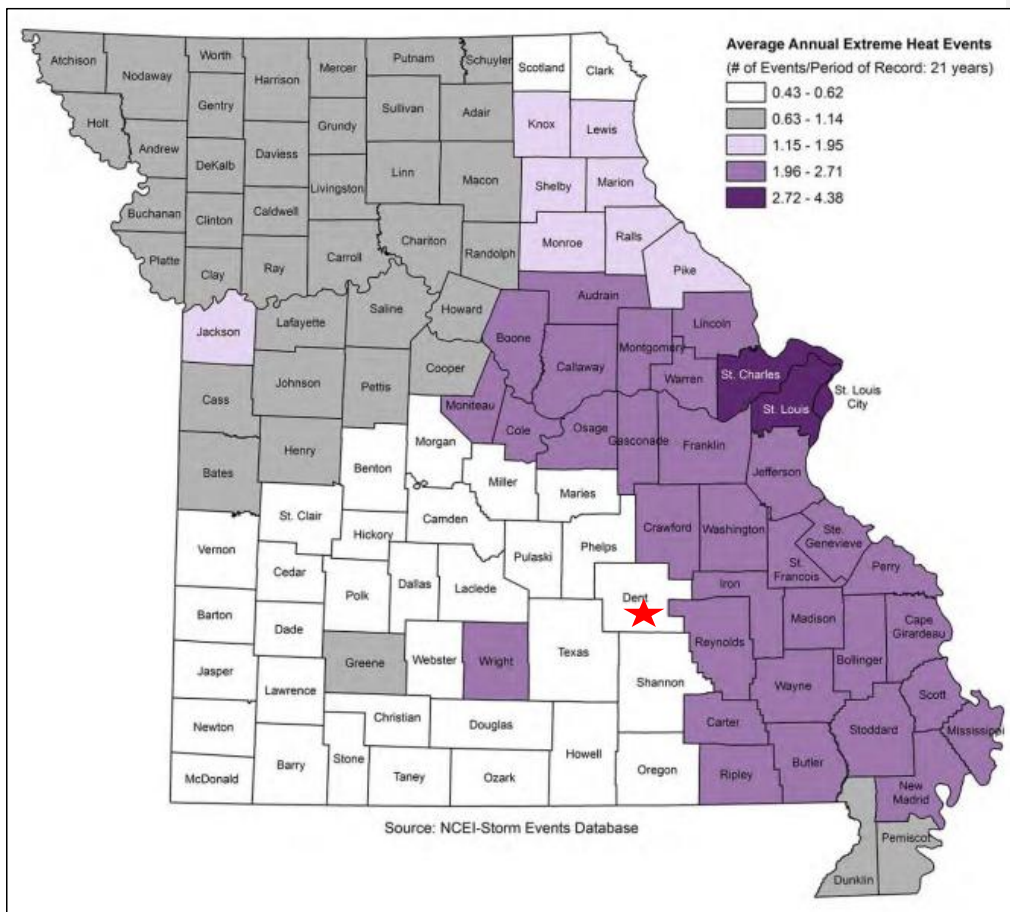
Figure 3.28. Average Annual Occurrence for Extreme Heat
