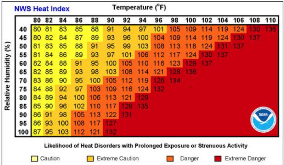
Figure 3.25. Heat Index (HI) Chart
