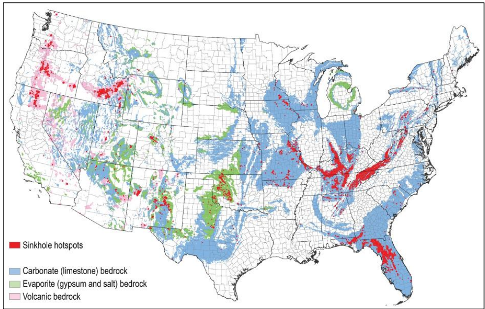
Figure 3.43. Karst Map of the Conterminous United States - 2020
